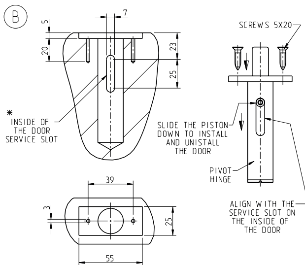
DRILING SCHEME FOR THE DOOR TOP HINGE + SCREWS 5X20 + SERVICE SLOT
